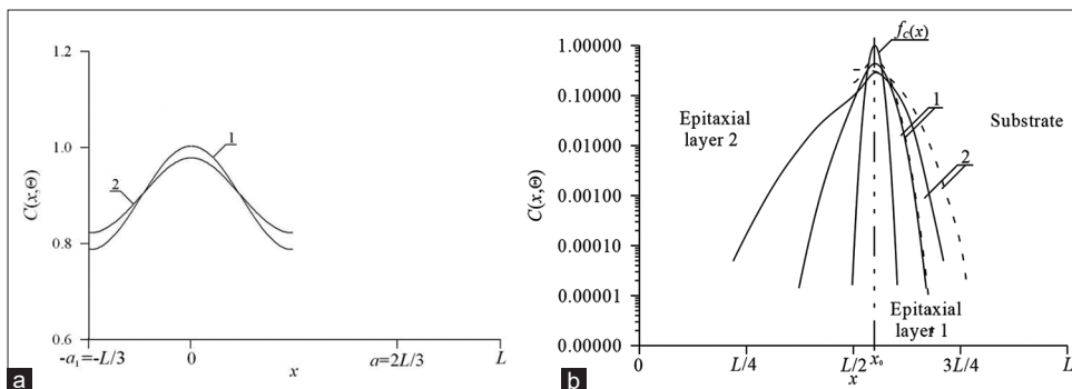
Figure 3: (a) Distributions of concentration of dopant, infused in average section of epitaxial layer of heterostructure from Figs. 1 in direction parallel to interface between epitaxial layer and substrate of heterostructure. Difference between values of dopant diffusion coefficients increases with increasing of number of curves. Value of dopant diffusion coefficient in this section is smaller, than value of dopant diffusion coefficient in nearest sections. (b) Calculated distributions of implanted dopant in epitaxial layers of heterostructure. Solid lines are spatial distributions of implanted dopant in system of two epitaxial layers. Dashed lines are spatial distributions of implanted dopant in one epitaxial layer. Annealing time increases with increasing of number of curves
